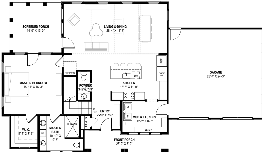
1ST FLOOR PLAN - 1,447 SF
