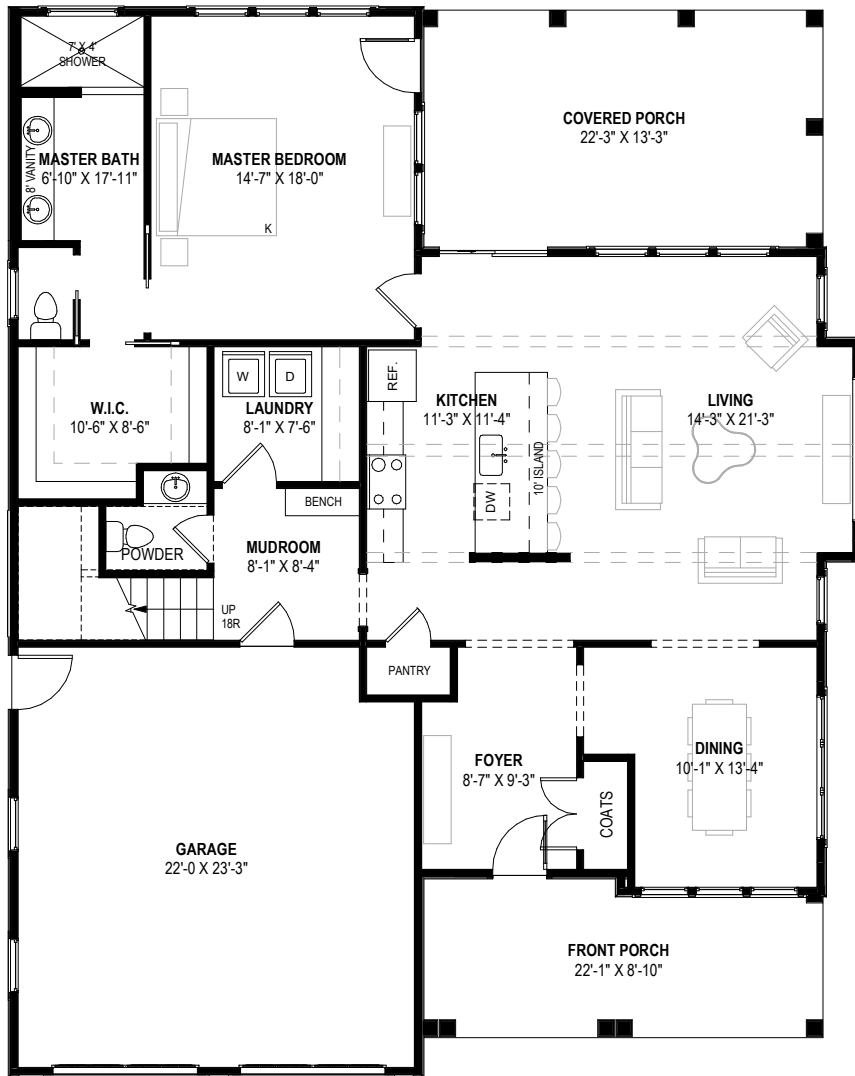
1ST FLOOR PLAN - 1,623 SF
