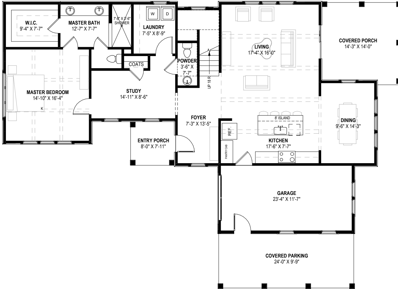
1ST FLOOR PLAN - 1,592 SF
