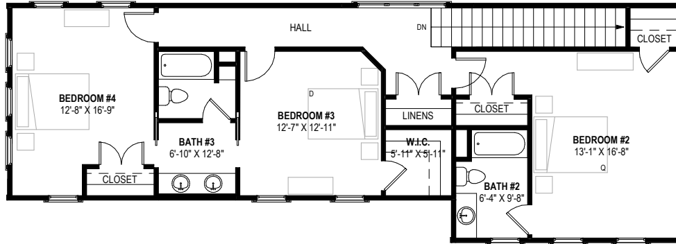
2ND FLOOR PLAN - 1,065 SF
